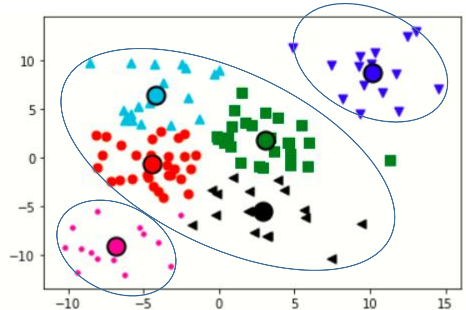
k-means (6 Clusters)
